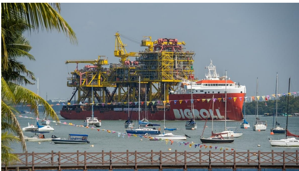
Topsides and bridges of Tyra Redevelopment Project sailed away from Sembcorp Marine Admiralty Yard on 25 July 2021
